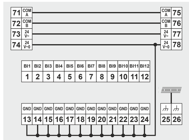
Fig. 17. CentralLine Panel Bus Binary Input Modules (schematic)
